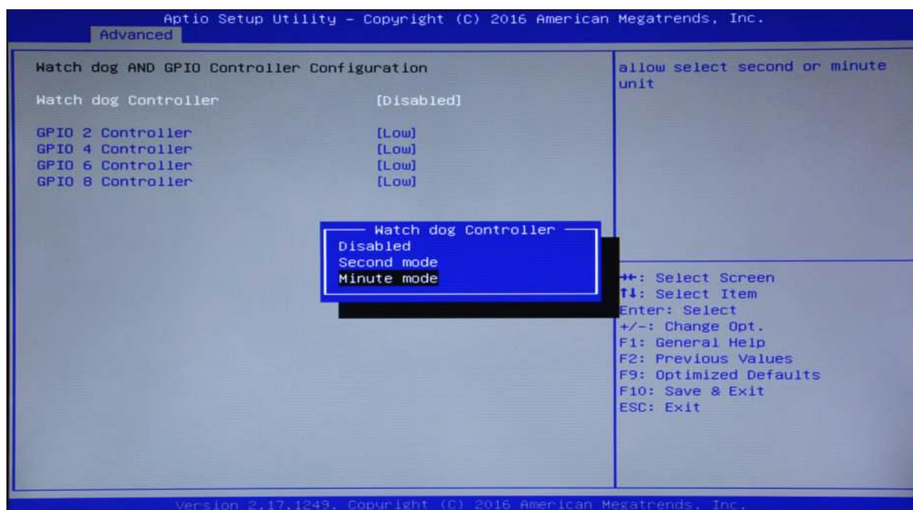
Рисунок 9. Watch dog AND GPIO Controller Configuration
